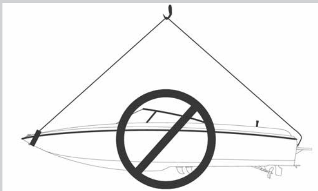
INCORRECT HOISTING
