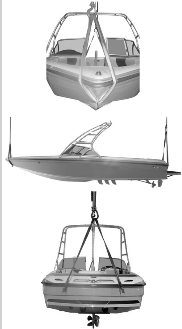
CORRECT HOISTING
