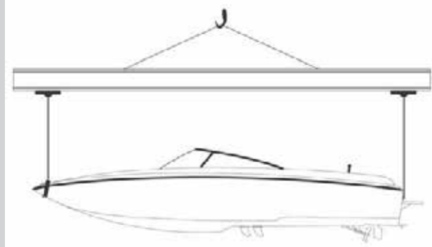
CORRECT HOISTING
